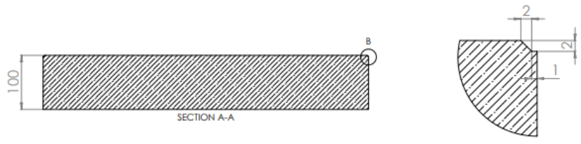
DETAIL B SCALE 5:1
